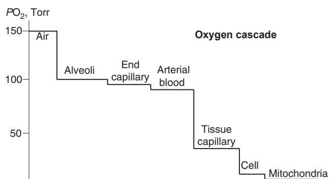
Figure 6 Oxygen cascade—the series of convective, diffusive, and biochemical barriers that progressively lower O 2 tension until it reaches the near-anoxic level necessary for optimal mitochondrial function within cells.
